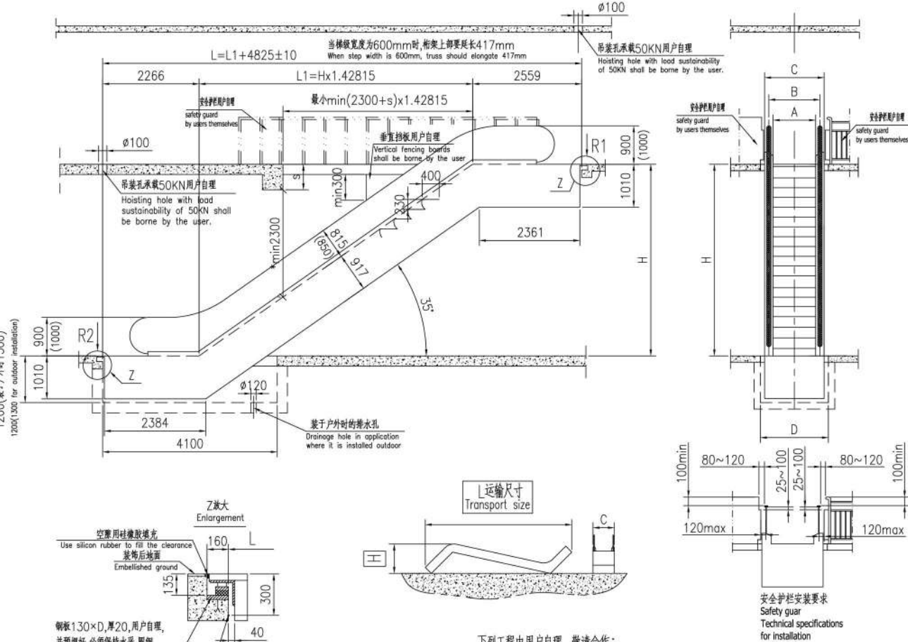
35° FPL Common Type/FML Slim Type Escalator Construction Layout
