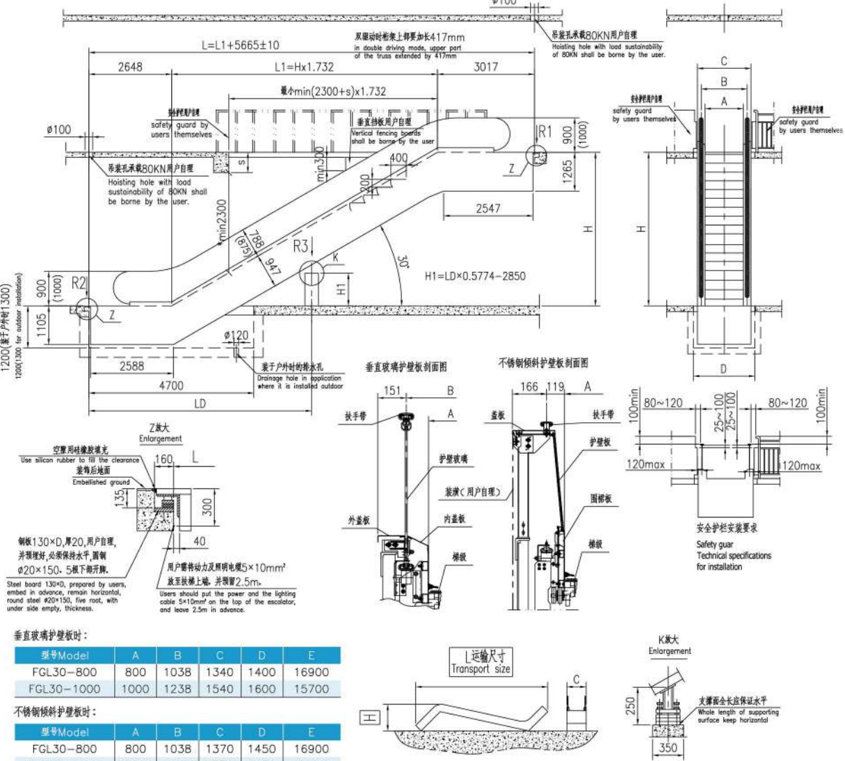
30°FGL Public Traffic Type Escalator Construction Layout
