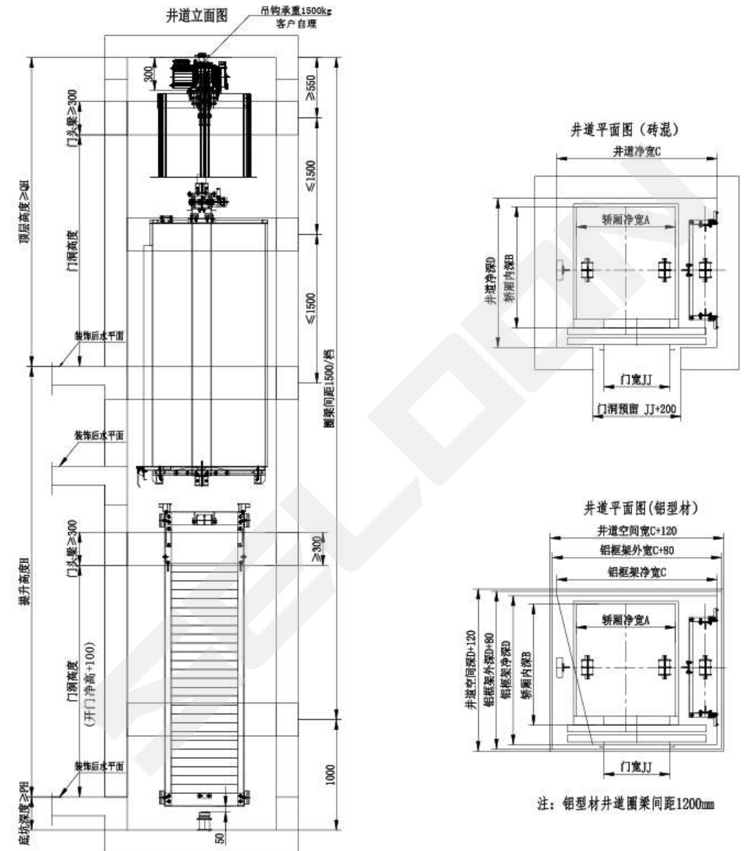
Side-placement steel band type home elevator construction layout chart
