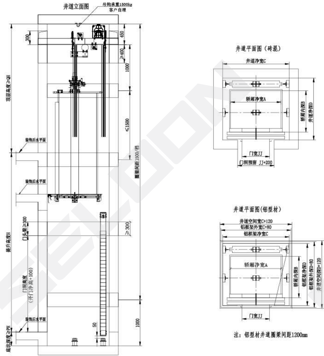
Rear placement steel band type home elevator construction layout chart
