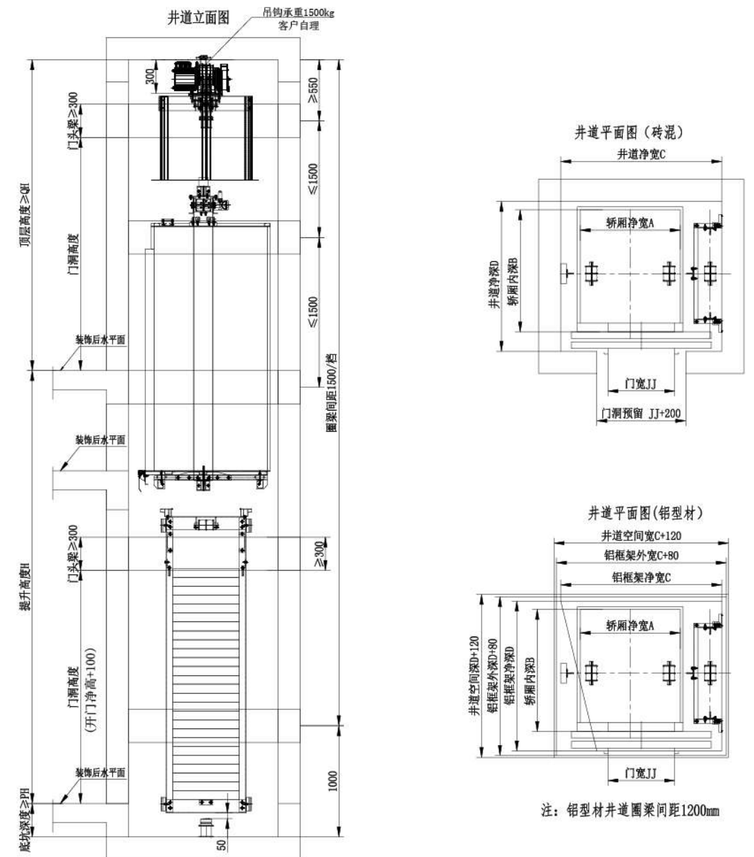
Side-placement steel band type home elevator construction layout chart
