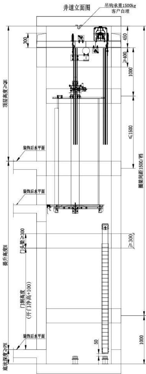
Rear placement steel band type home elevator construction layout chart
